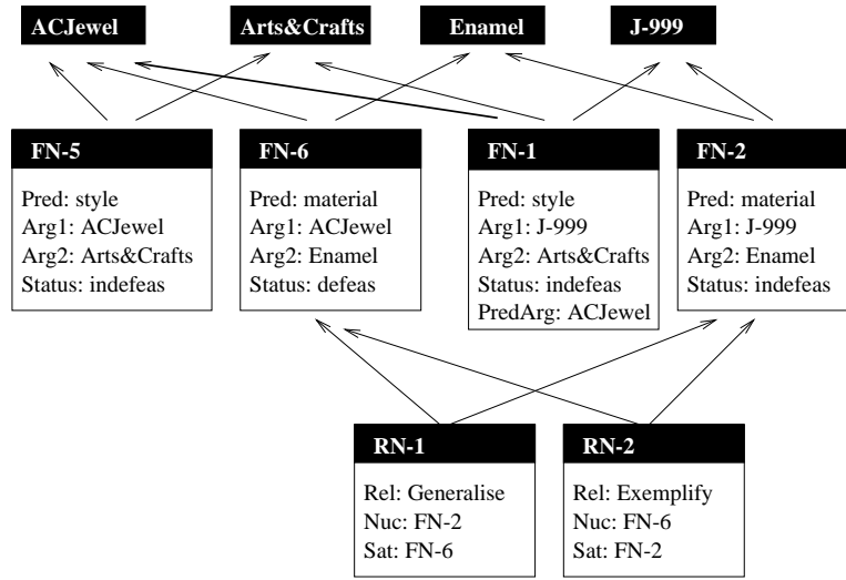
Fig. 13. Relations arising from Generalisations
